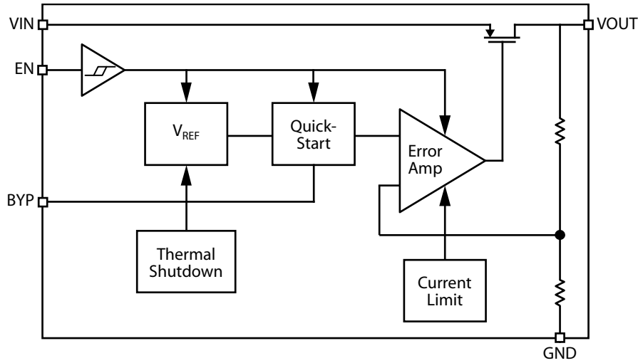
MIC5305 Block Diagram - Fixed
