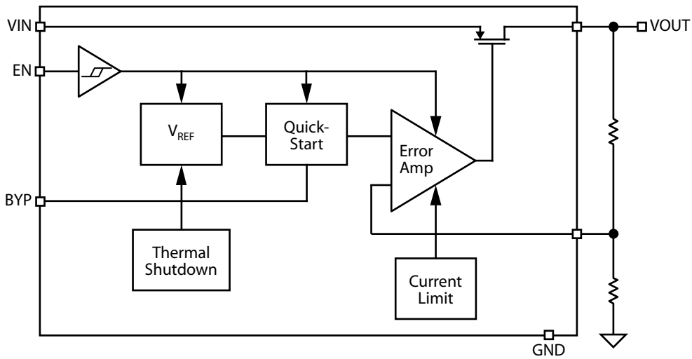
MIC5305 Block Diagram - Adjustable
