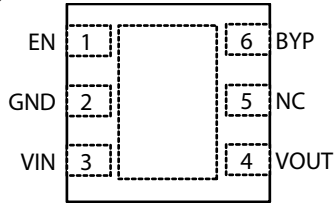
MIC5305-x.xBML 6-Pin 2mm × 2mm MLF™ (ML) (Top View)
