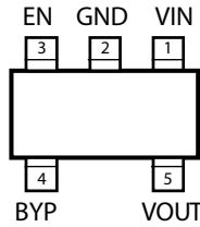
MIC5305-x.xBD5 TSOT-23-5 (D5) (Top View)
