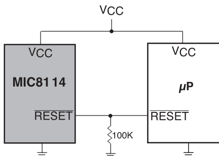
Figure 3. RESET Valid to V_{CC} = 0V .
