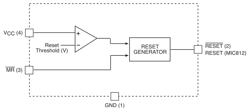
Figure 1. MIC811/812 Block Diagram
