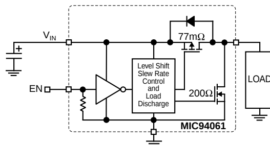
Load Switch Application with Capacitive Load Discharge
