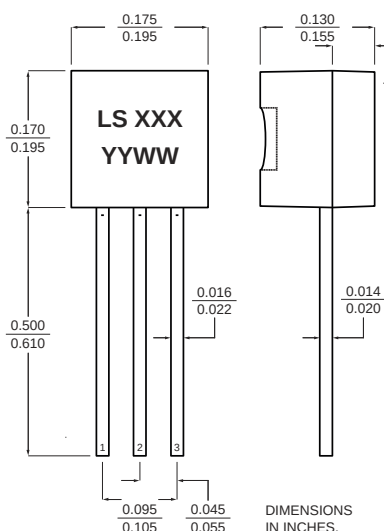
TO-92
