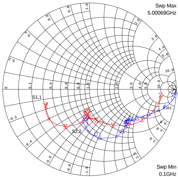
Smith Chart
