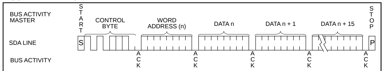
FIGURE 4-2: PAGE WRITE
