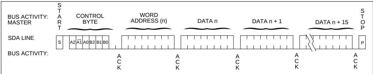
FIGURE 4-2: PAGE WRITE
