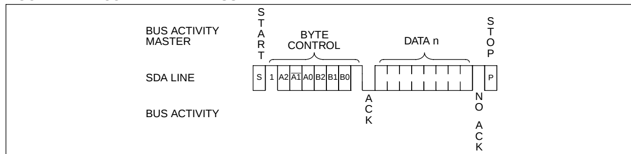
FIGURE 7-2: RANDOM READ
