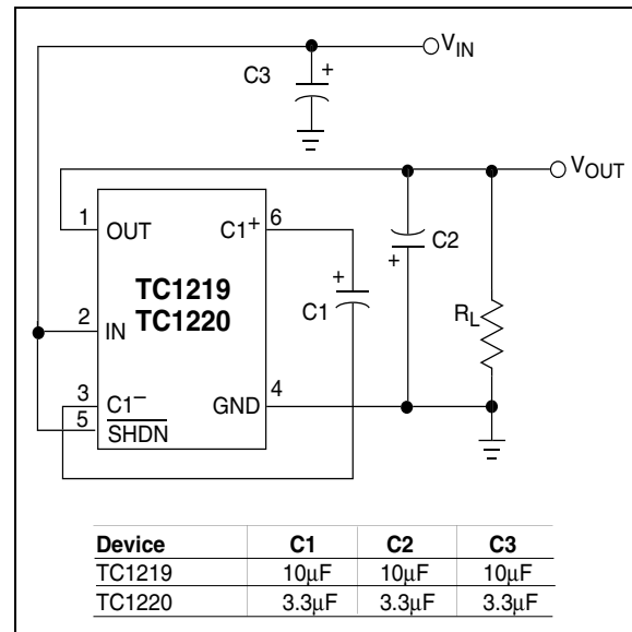
FIGURE 4-3: VOLTAGE INVERTER TEST CIRCUIT
