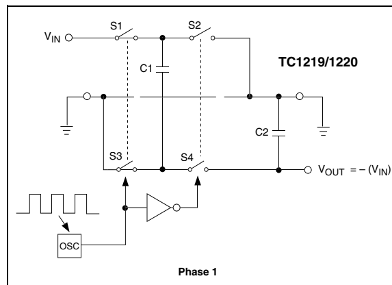
FIGURE 3-1: IDEAL SWITCHED CAPACITOR CHARGE PUMP
