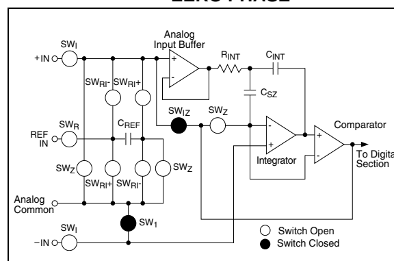
FIGURE 3-5: INTEGRATOR OUTPUT ZERO PHASE
