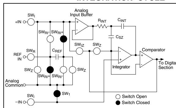
FIGURE 3-4: REFERENCE VOLTAGE INTEGRATION CYCLE
