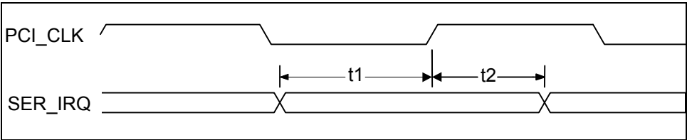
Figure 13.20 - Setup and Hold Time
