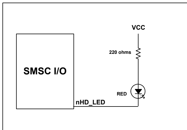
Figure 7.6 - NHD_LED Circuit
