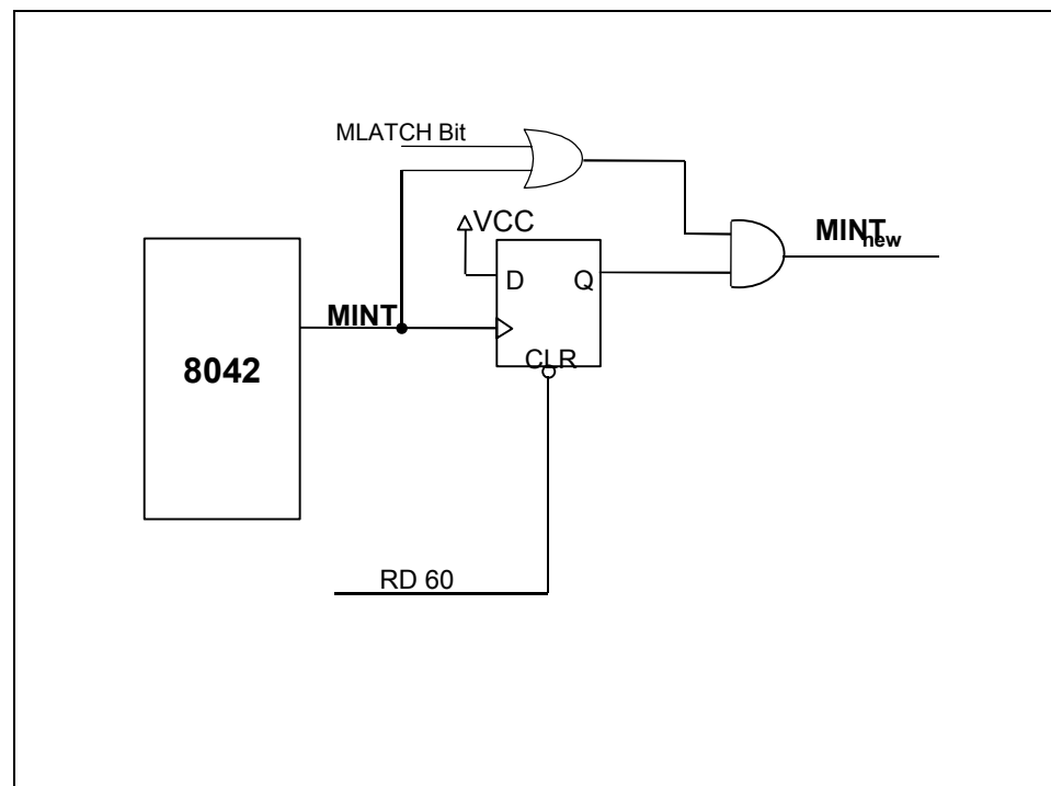
Figure 7.3 - Mouse Latch
