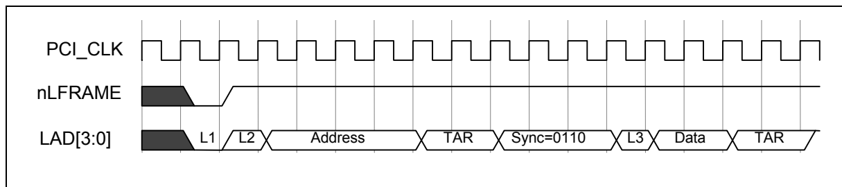
Figure 13.8 - I/O Read
