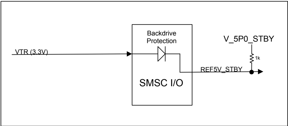
Figure 7.9 - REF5V_STBY
