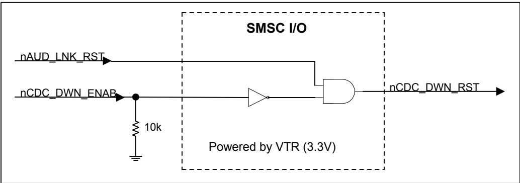
Figure 7.21 - CNR Circuit
