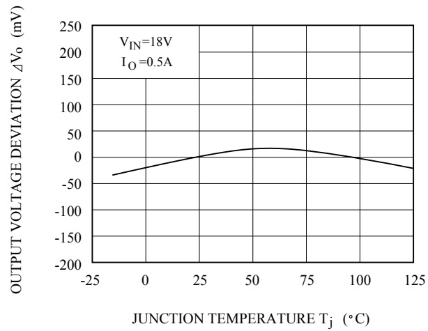
Fig.5-4 T_j - \Delta V_O (KIA278R12)
