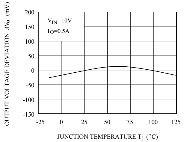
Fig.5-2 T_j - \Delta V_O (KIA278R08)
