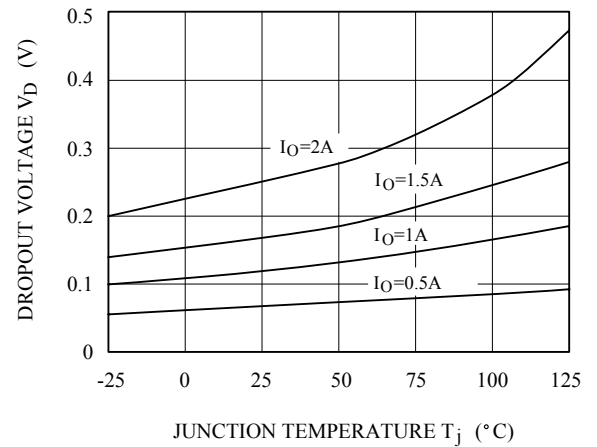
Fig.8 T_j - V_D
