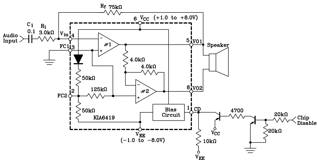
FIGURE26-SPLIT SUPPLY OPERATION
