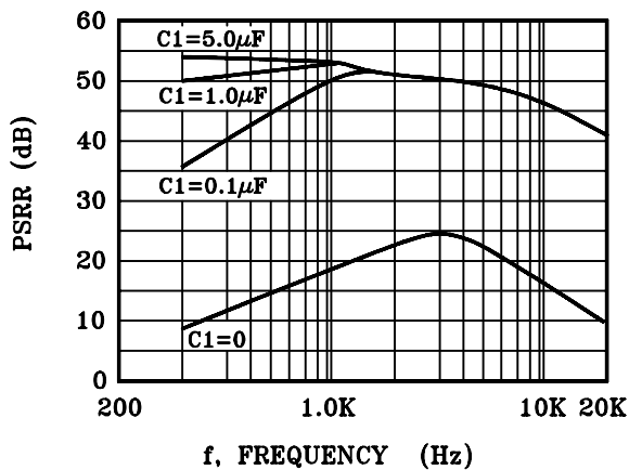
FIGURE6-C2=1.0 \mu F
