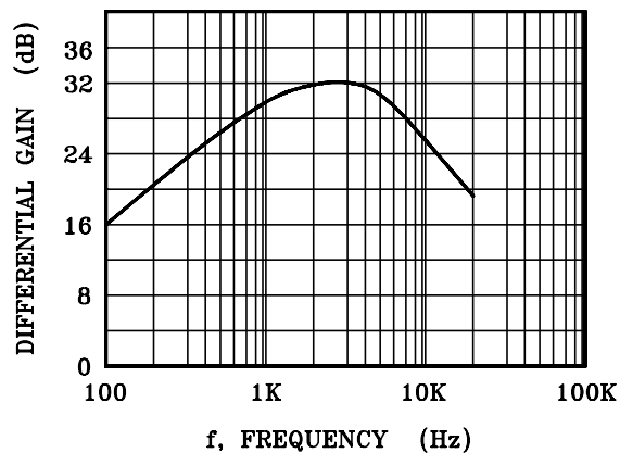
FIGURE25-FREQUENCY RESPONSE OF FIGURE24
