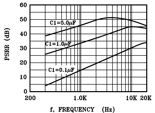
FIGURE7-C2=0
