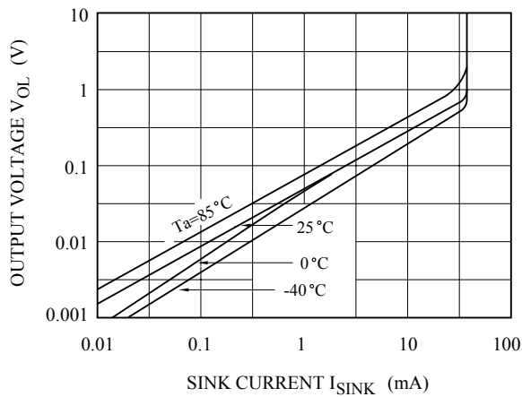
V_{OL} - I_{SINK}
