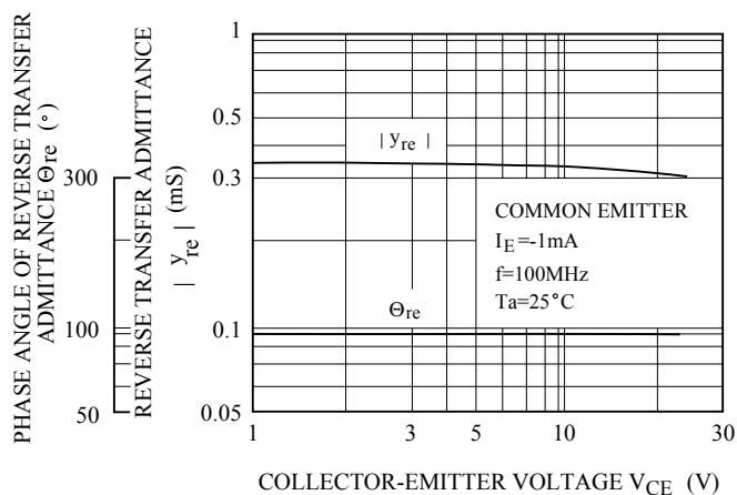
|y_{re}|, \theta_{re} - V_{CE}
