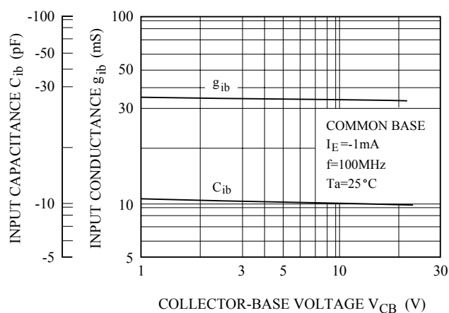
C_{ib}, g_{ib} - V_{CB}
