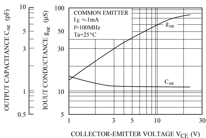
C_{oe}, g_{oe} - V_{CE}
