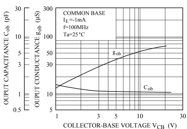
C_{ob}, g_{ob} - V_{CB}
