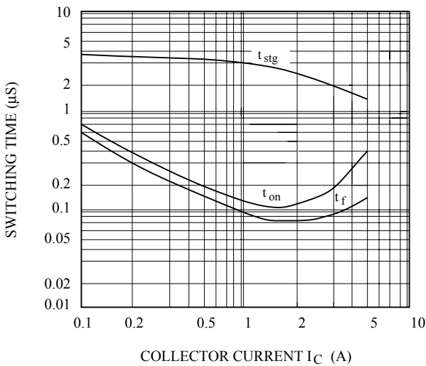
SWITCHING CHARACTERISTICS
