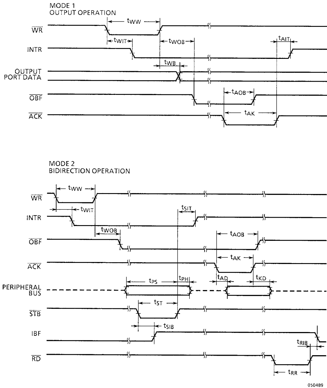
Figure 7.2 Timing diagram
