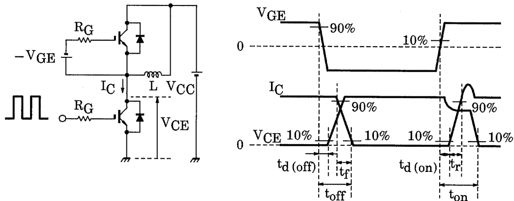
Switching loss measurement waveforms
