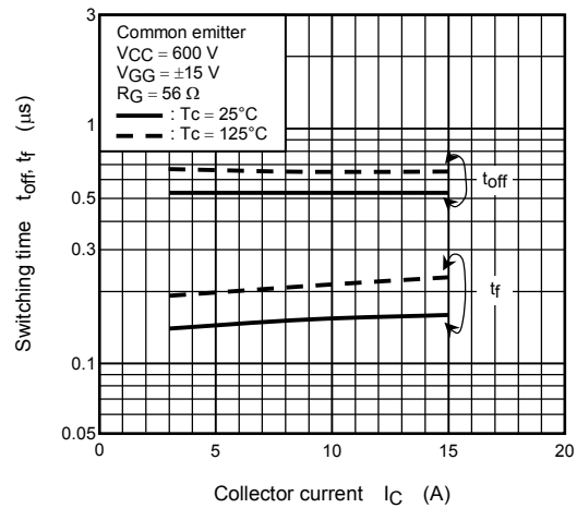
Switching time t_{off}, t_f - I_C
