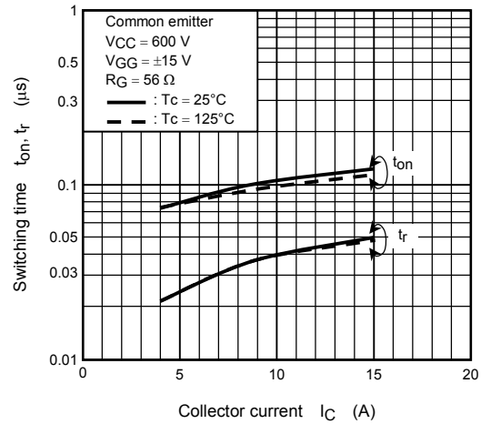
Switching time t_{on}, t_r - I_C
