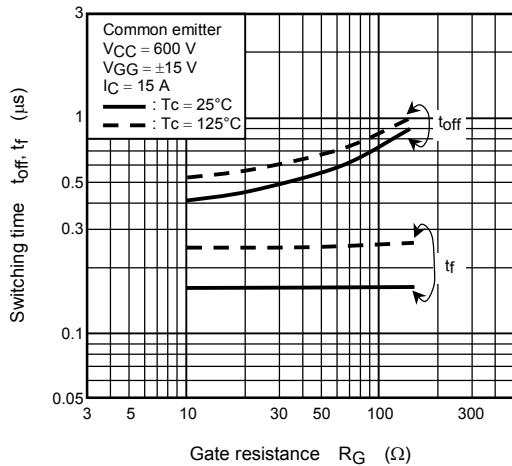
Switching time t_{off}, t_f - R_G
