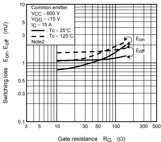
Switching loss E_{on}, E_{off} - R_G
