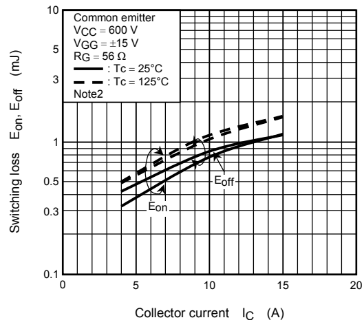
Switching loss E_{on}, E_{off} - I_C
