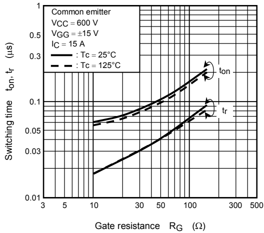
Switching time t_{on}, t_r - R_G
