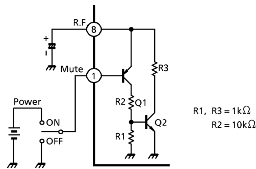
Fig.4 Mute circuit
