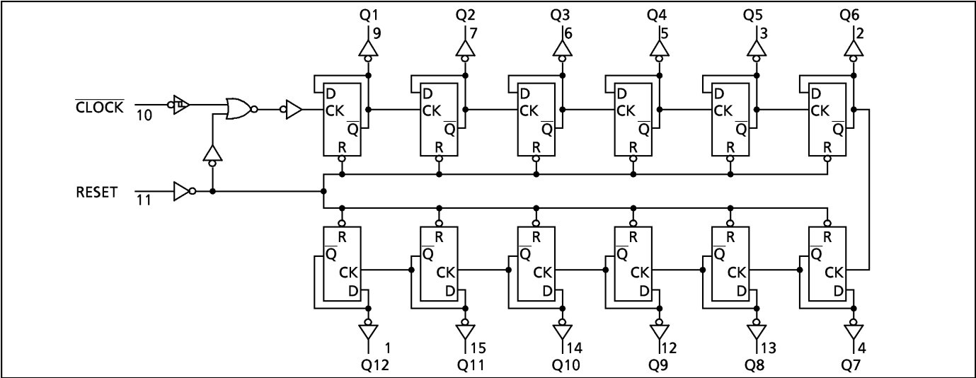
LOGIC DIAGRAM
