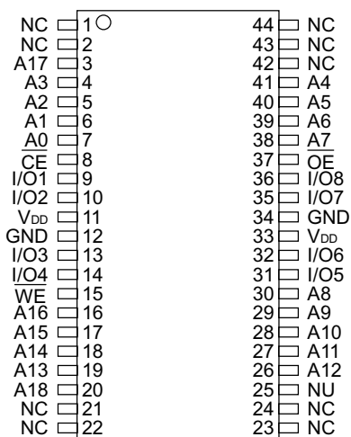
(TC55V8512FT)
