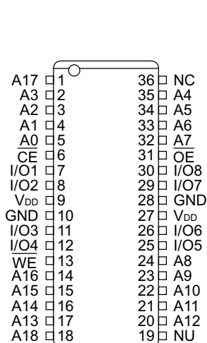
(TC55V8512J)
