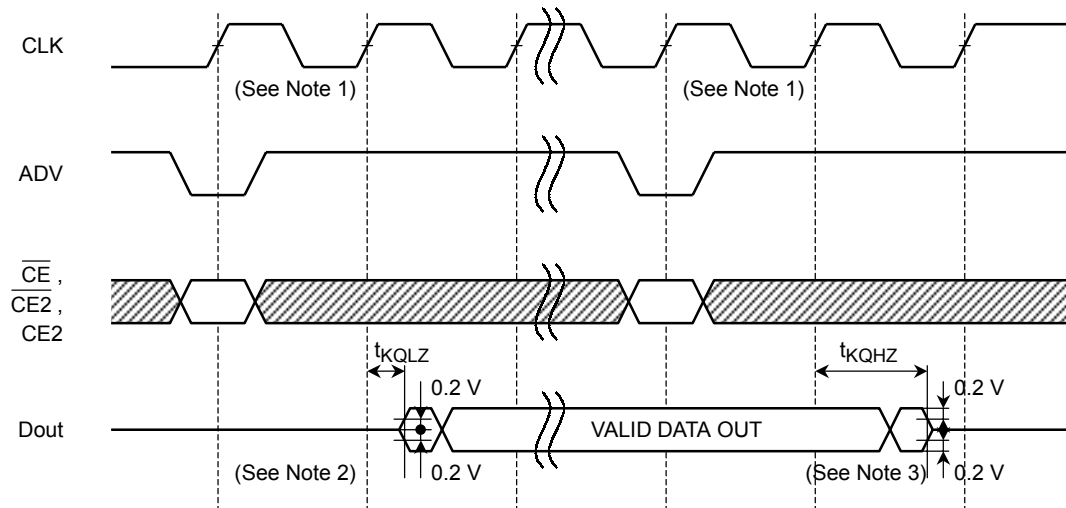
(A) t_{KQLZ} , t_{KQHZ}
