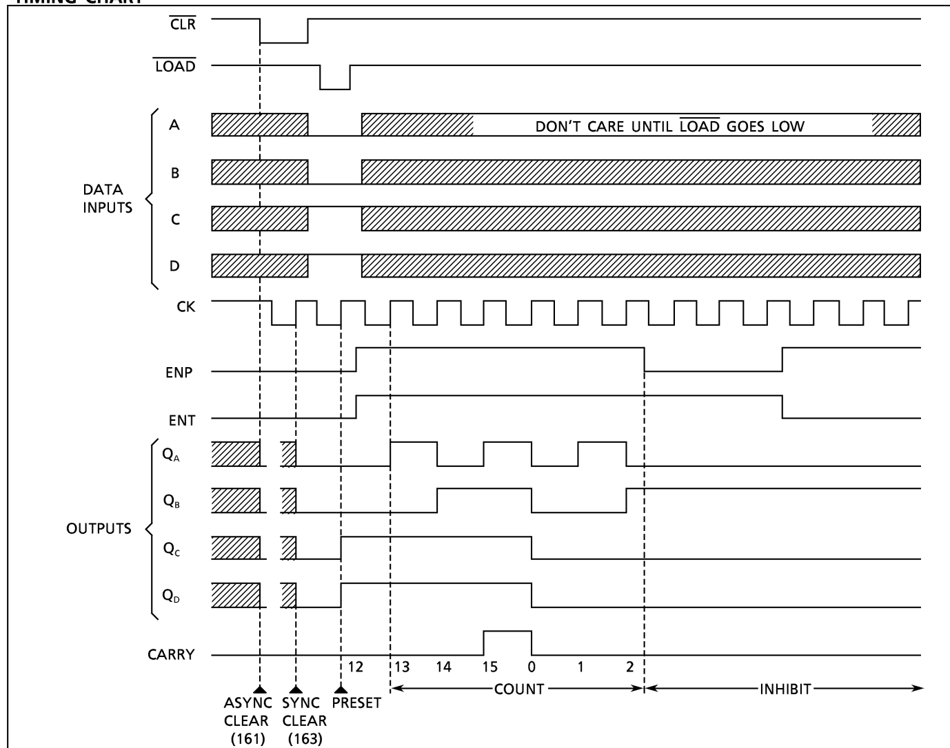
TIMING CHART
