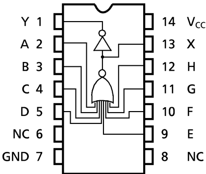
(TOP VIEW) NC:No Connection
