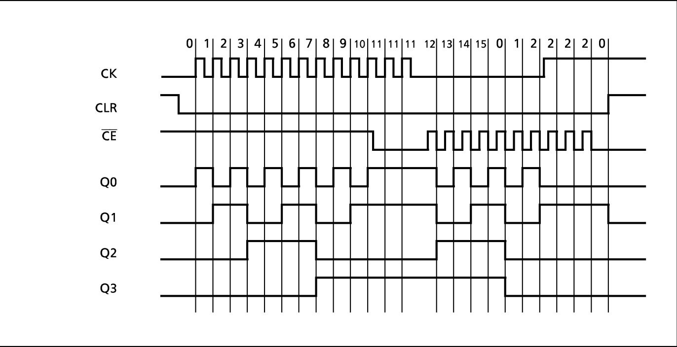
TIMING CHART
