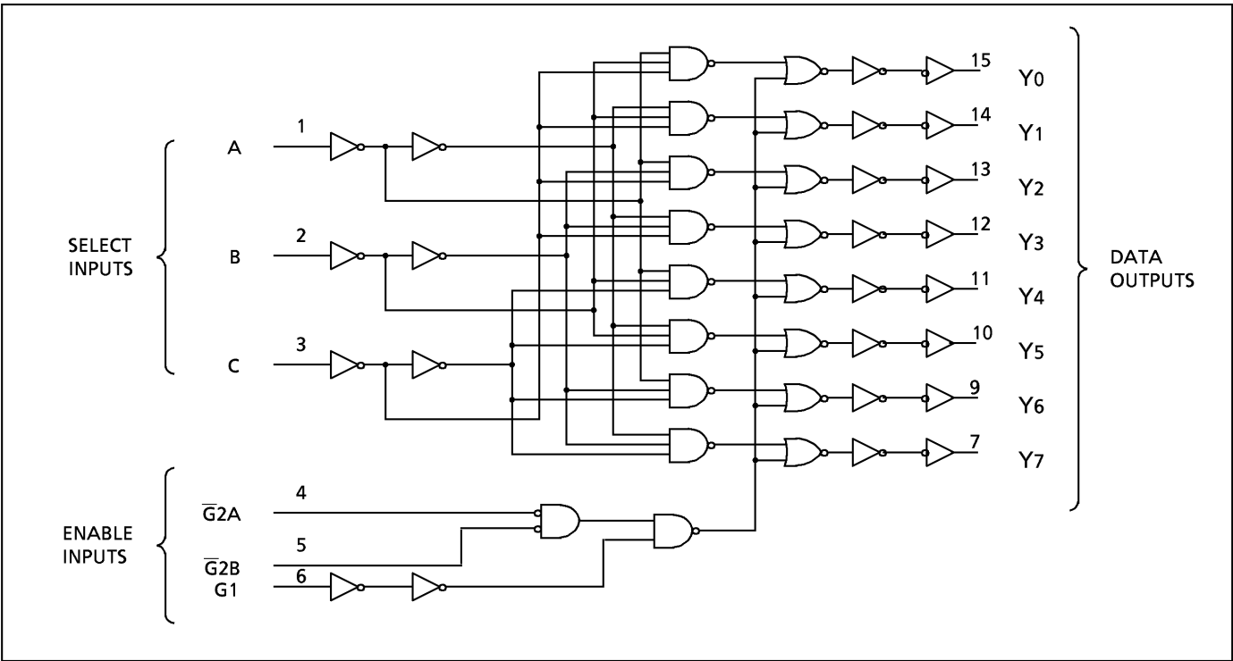
LOGIC DIAGRAM
