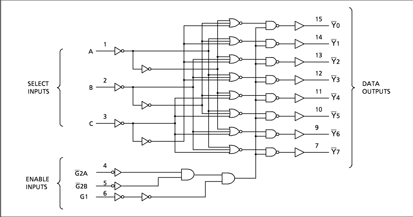
SYSTEM DIAGRAM
