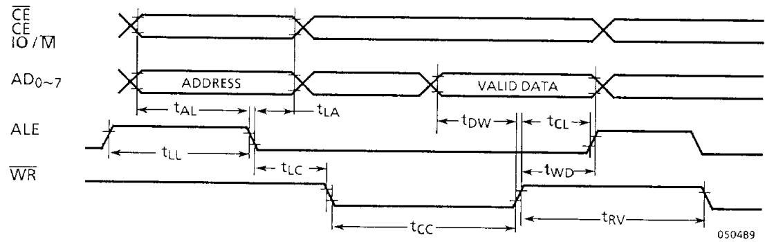
Figure 8.2 WRITE CYCLE
