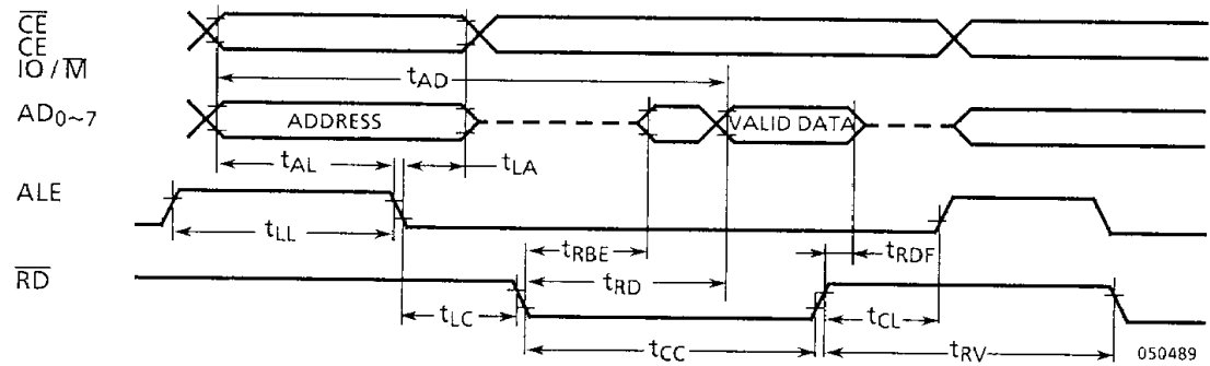
Figure 8.1 READ CYCLE
