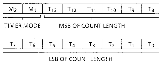
Figure 6.3 Timer Format
