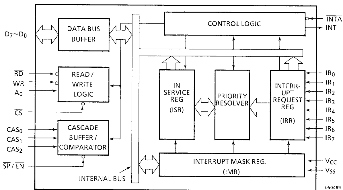
Figure 4.1 BLOCK DIAGRAM
