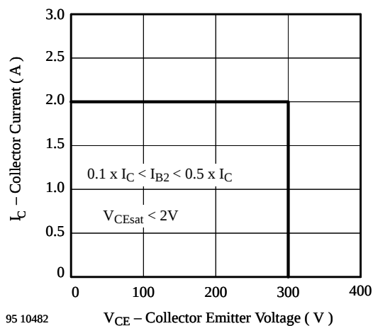
Figure 4. V_{\text{CEW}} - Diagram
