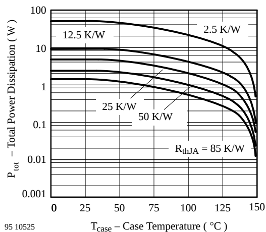
Figure 7. P_{\text{tot}} vs. T_{\text{case}}
