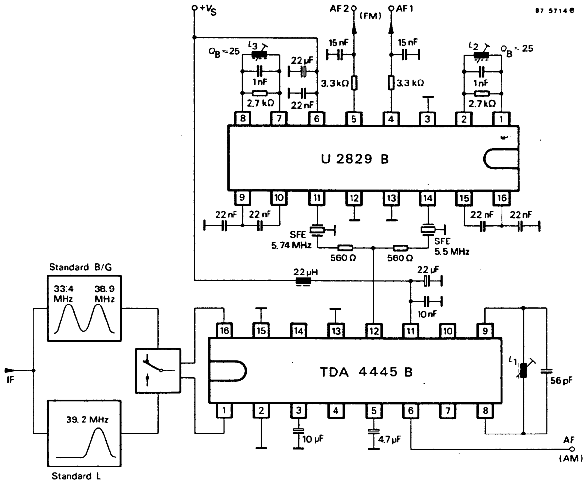
Figure 4. Bistandard operation
