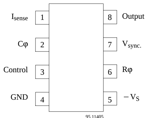
Figure 3. Pinning
