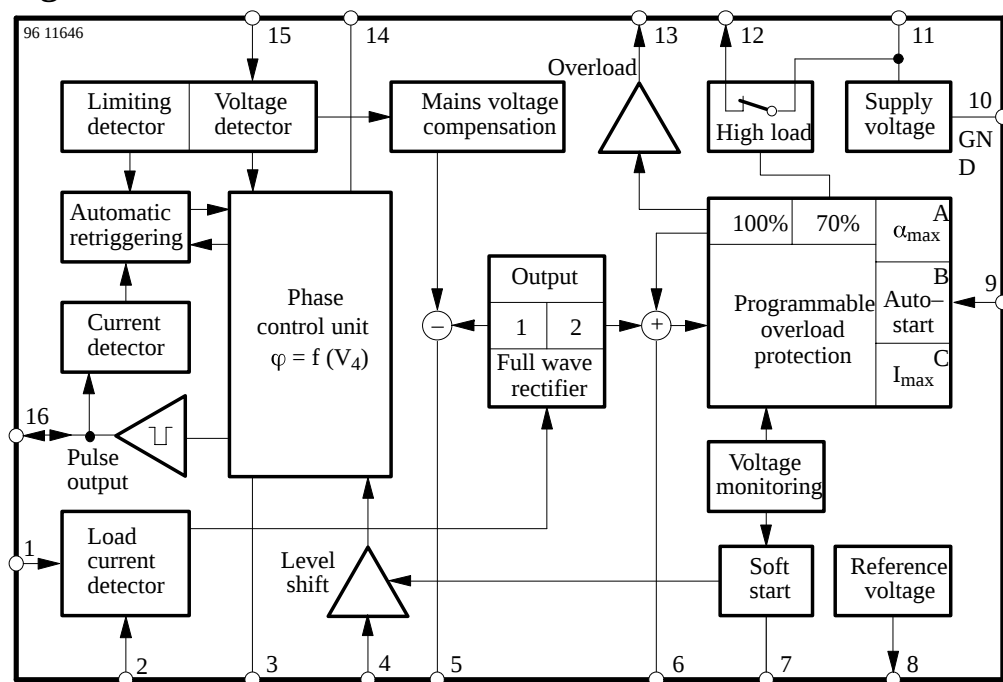
Figure 1. Block diagram
