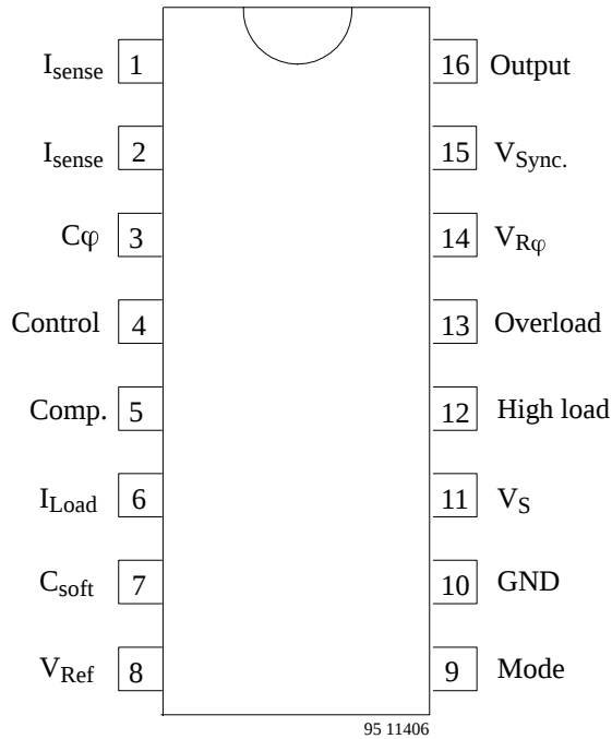
Figure 3. Pinning
