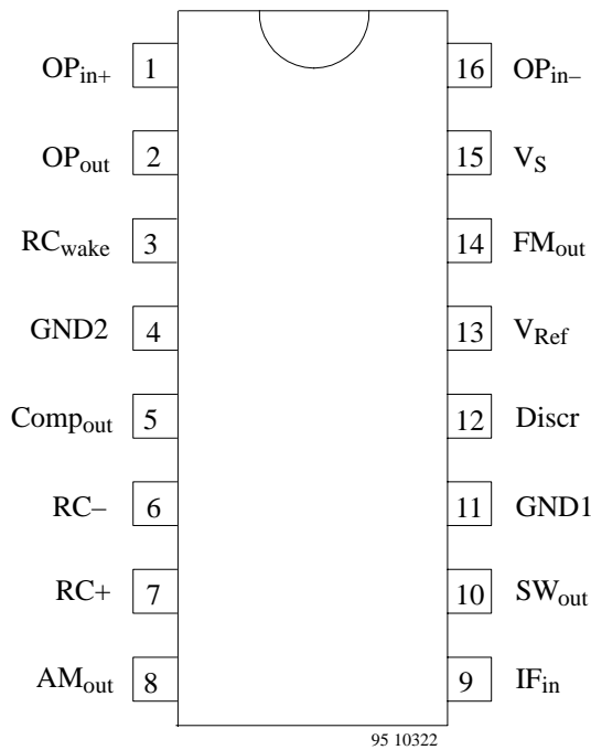
Figure 2. Pin description
