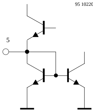
Figure 5. Pin 5 IF_{in}
