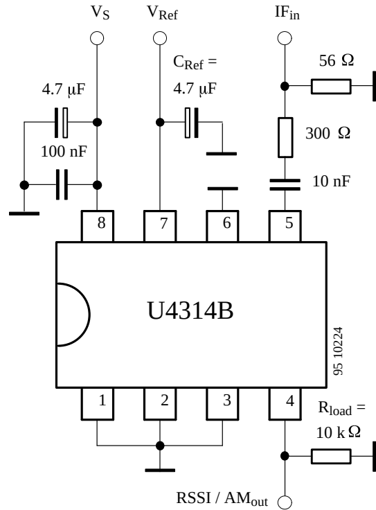
Figure 8. Test circuit
