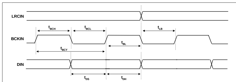
Figure 4 Audio Data Input Timing
