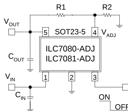
Figure 3: Application circuit for adjustable output voltage
