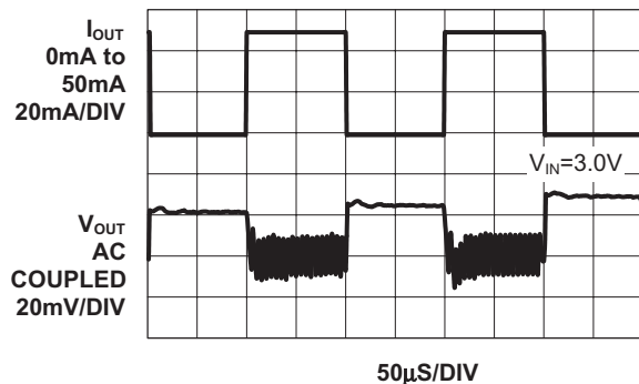
Load Transient Response for 50mA AAT3110-5
