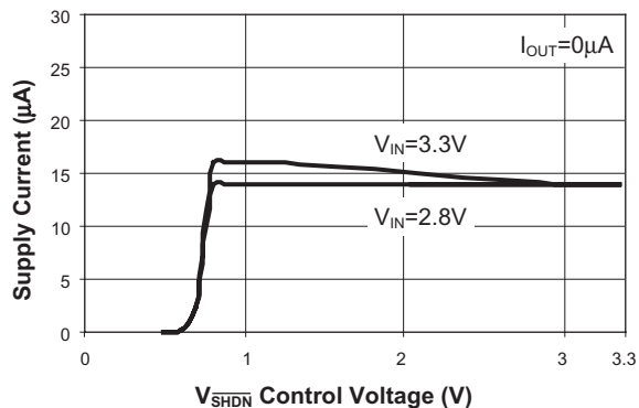
Supply Current vs. V_{SHDN} AAT3110-3.3
