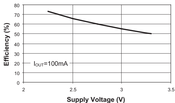
Efficiency vs. Supply Voltage AAT3110-3.3
