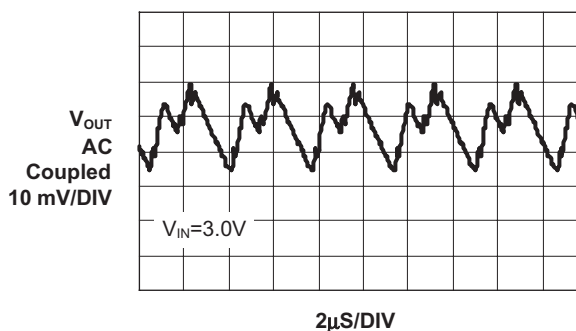
Output Ripple with I_{OUT}=100 mA AAT3110-5
