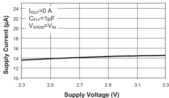
Supply Current vs. Supply Voltage AAT3110-3.3
