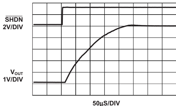
Startup Time with 50 mA Load AAT3110-5
