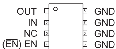
AAT3221 SC70JW-8 (Top View)
