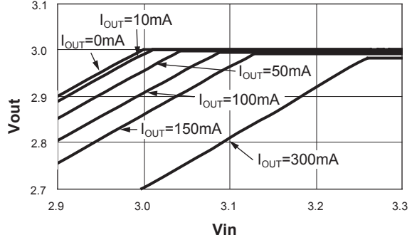
Dropout Characteristics
