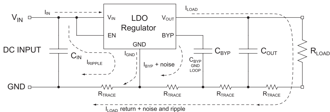
Figure 18: Common LDO Regulator Layout with C_{\text{BYP}} Ripple feedback loop
