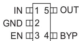
SOT-23-5 (Top View)
