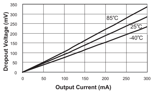
Dropout Voltage vs. I_{OUT}
