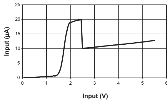
Quiescent Current
