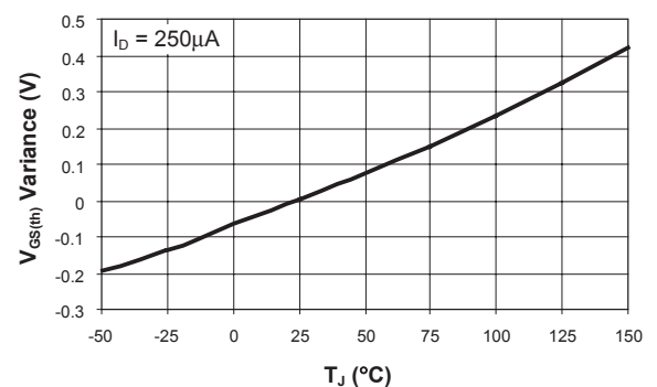
Threshold Voltage
