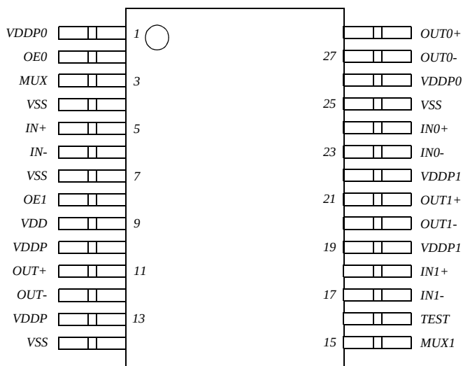
Figure 3: Pin Diagram
