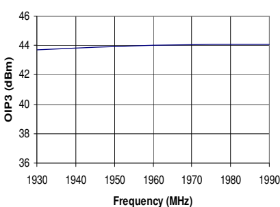
OIP3 vs. Frequency
