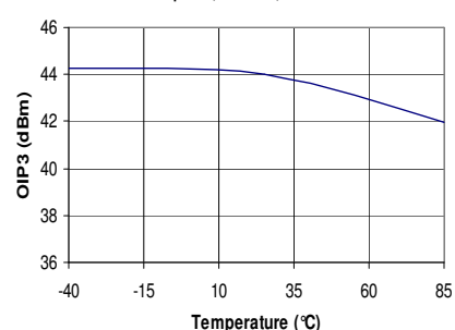
OIP3 vs. Temperature
