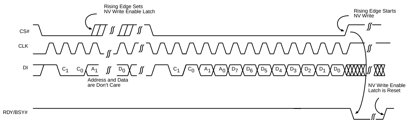
FIGURE 2. WRITE SEQUENCE
