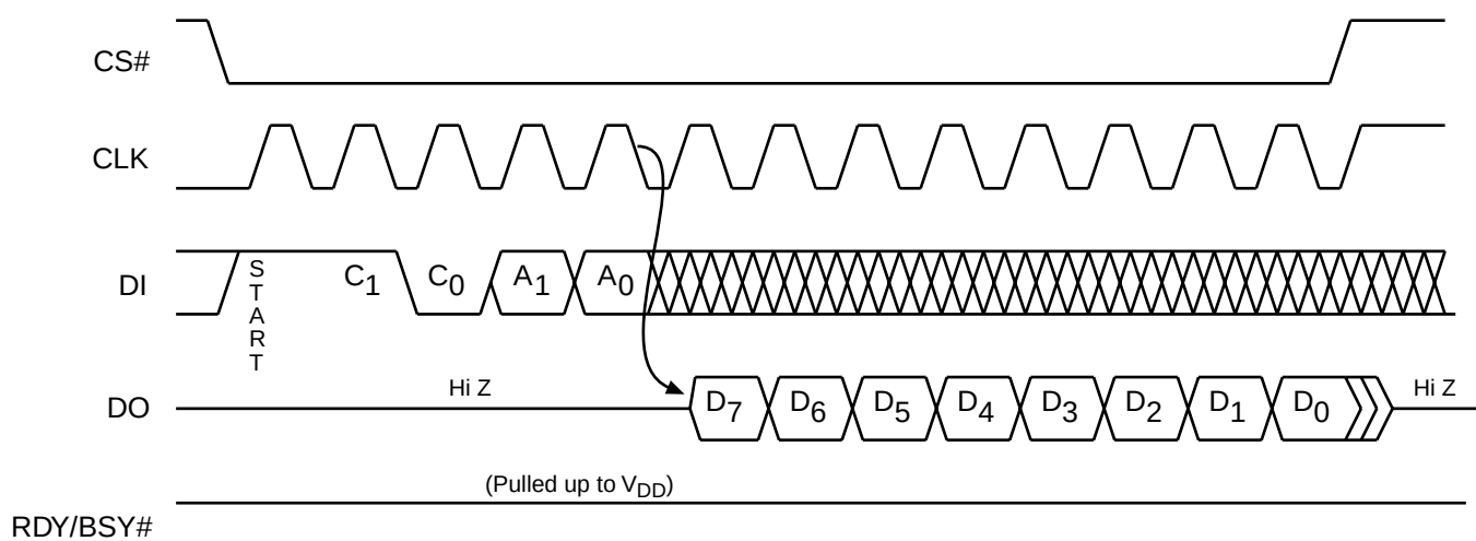
FIGURE 1. READ SEQUENCE
