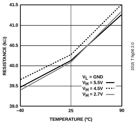
FIGURE 6. VL to VH END-TO-END RESISTANCE OVER TEMPERATURE
