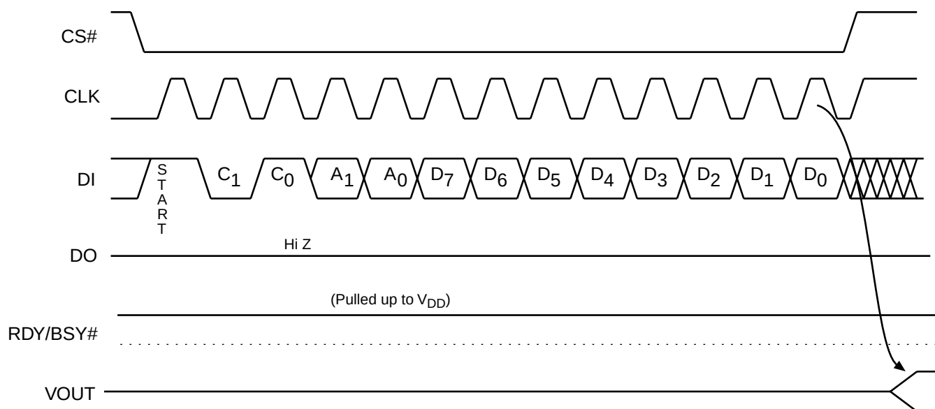
FIGURE 2. WRITE SEQUENCE
