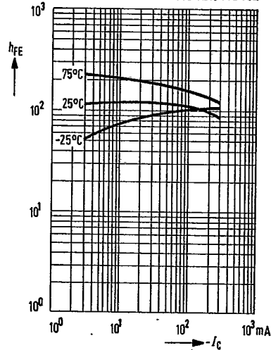
DC current gain h_{\text{FE}} = f(I_{\text{C}}) -V_{\text{CE}} = 0.5 \text{ V}; T_{\text{amb}} = \text{parameter} (common emitter configuration)
