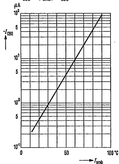
Collector cutoff current versus temperature I_{CBO} = f(T_{amb}) ; -V_{CE} = 20V
